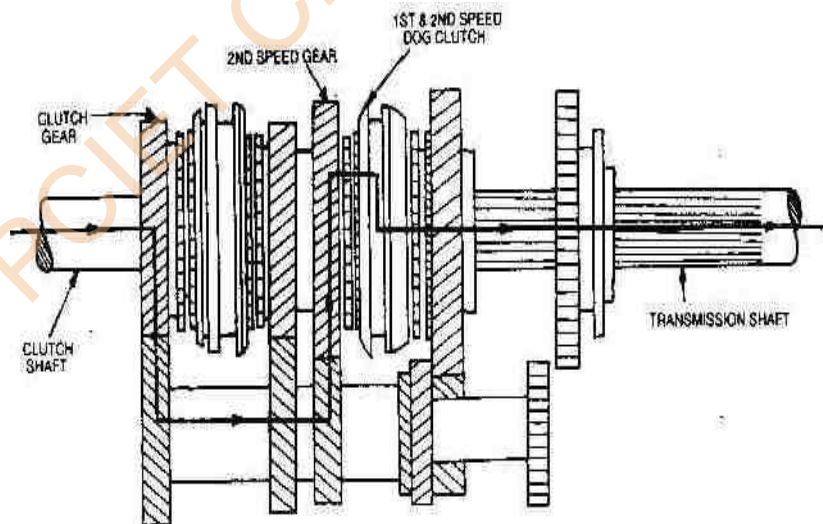
Fig. 23.21. Second gear.
